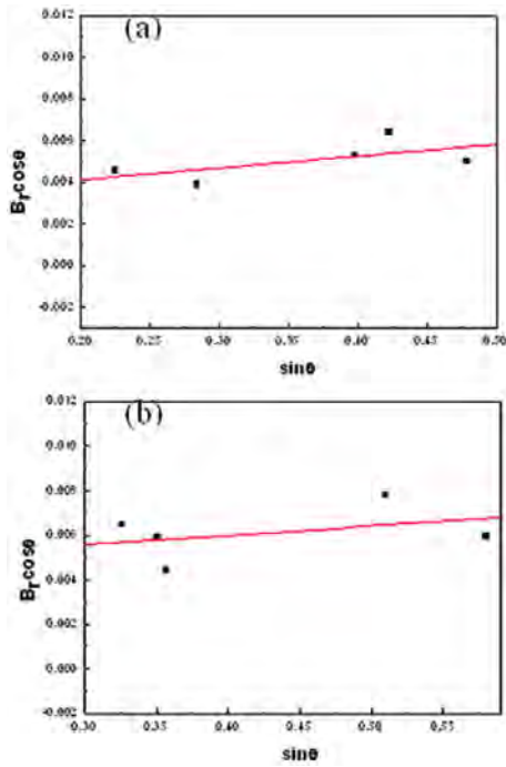
Fig. 7. Plot of B_r(B_{\text{crystalline}} + B_{\text{strain}}) \cos\theta versus \sin\theta for \text{Mg}_2\text{Al}_6\text{Ti}_7\text{O}_{25} (a) and \text{Mg}_{0.6}\text{Al}_{0.8}\text{Ti}_{1.6}\text{O}_5 (b) in composite sintered from the 7.6\text{TiO}_2 + 3.4\text{Al}_2\text{O}_3 + 2.6\text{MgO} powders milled for 10 h.
