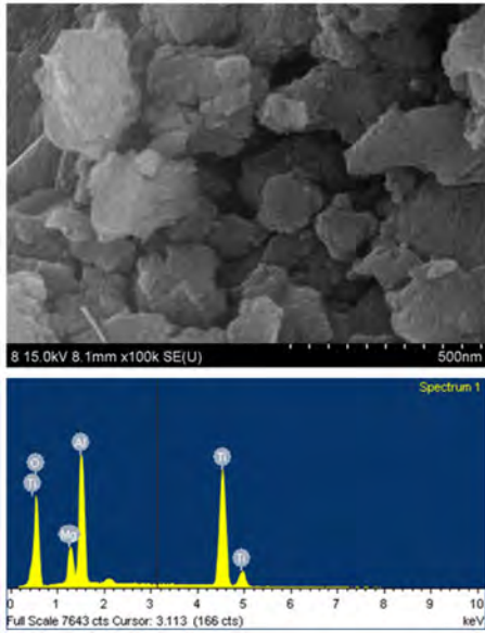
Fig. 4. FE-SEM image of the \text{TiO}_2 , \text{Al}_2\text{O}_3 and \text{MgO} powders milled for 10 h.
