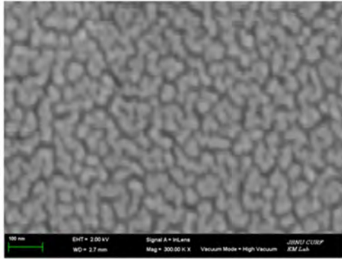
Fig. 8. FE-SEM image of sintered \text{Mg}_2\text{Al}_6\text{Ti}_7\text{O}_{25}\text{-Mg}_{0.6}\text{Al}_{0.8}\text{Ti}_{1.6}\text{O}_5 composite.
