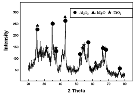
Fig. 2. X-ray diffraction patterns of the \text{TiO}_2 , \text{Al}_2\text{O}_3 and \text{MgO} powders milled for 10 h.
