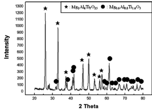
Fig. 6. XRD pattern of specimen of sintered \text{Mg}_2\text{Al}_6\text{Ti}_7\text{O}_{25} - \text{Mg}_{0.6}\text{Al}_{0.8}\text{Ti}_{1.6}\text{O}_5 composite from the high energy ball milled 7.6\text{TiO}_2 + 3.4\text{Al}_2\text{O}_3 + 2.6 \text{MgO} powders.
