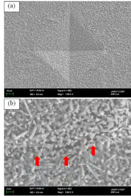
Fig. 9. Vickers indentation (a) and crack propagating (b) in the \text{Mg}_2\text{Al}_6\text{Ti}_7\text{O}_{25}\text{-Mg}_{0.6}\text{Al}_{0.8}\text{Ti}_{1.6}\text{O}_5 composite sintered from milled 7.6\text{TiO}_2 + 3.4\text{Al}_2\text{O}_3 + 2.6\text{MgO} powders.
