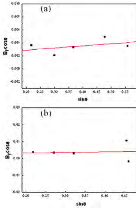
Fig. 3. Plot of B_r(B_{\text{crystalline}} + B_{\text{strain}}) \cos\theta versus \sin\theta for \text{Al}_2\text{O}_3 (a), and \text{TiO}_2 (b) powder milled for 10 h.
