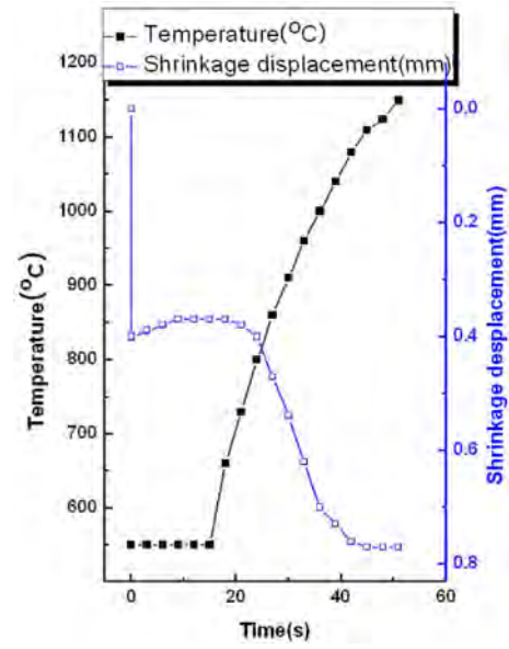
Fig. 5. Variations of temperature and shrinkage with heating time during the synthesis and sintering of 7.6\text{TiO}_2 + 3.4\text{Al}_2\text{O}_3 + 2.6 \text{MgO} powders milled for 10 h.
